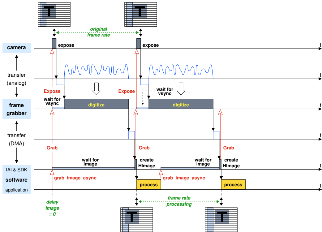
Figure 11: Using an asynchronously resettable camera together with grab_image_async (configuration as in figure 8 on page 23).
