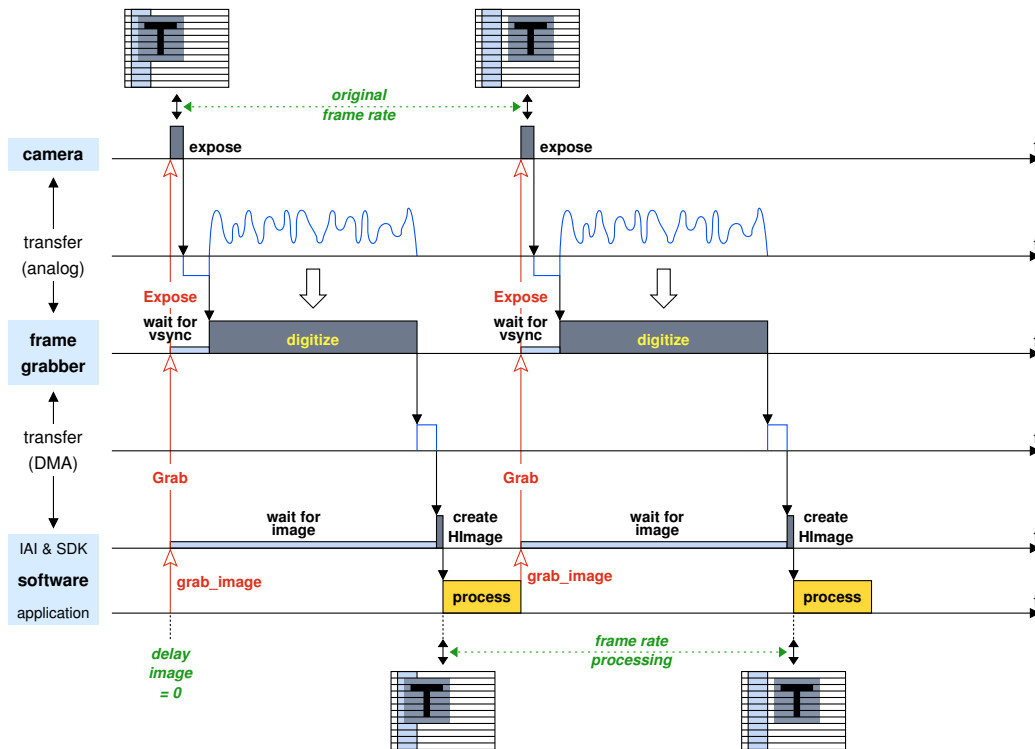
Figure 8: Using an asynchronously resettable camera together with grab_image (configuration: progressive-scan camera, frame grabber with burst transfer, volatile grabbing).
