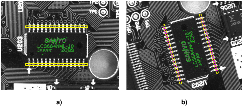
Figure 3.17: (a) Model image with measurement ROIs; (b) measuring the leads in the aligned ROIs.
