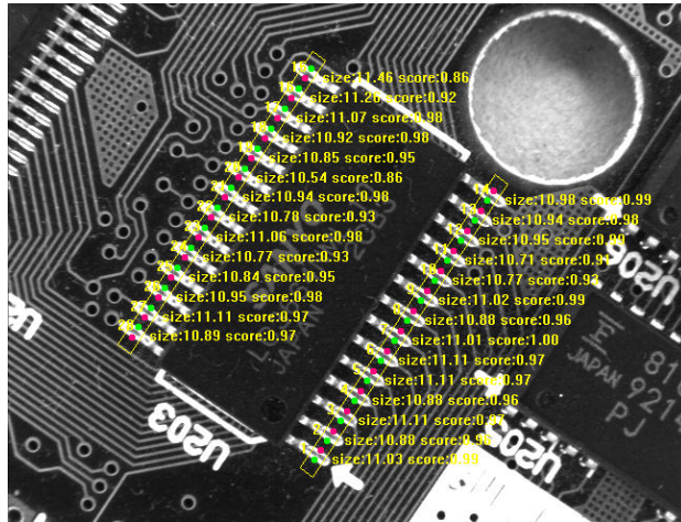
Figure 3.16: Measuring the width and distance of the leads.
