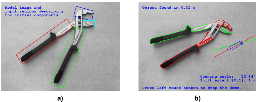
Figure 3.9: (a) Model image with specified ROIs for the components; (b) located pipe wrench in another state.
