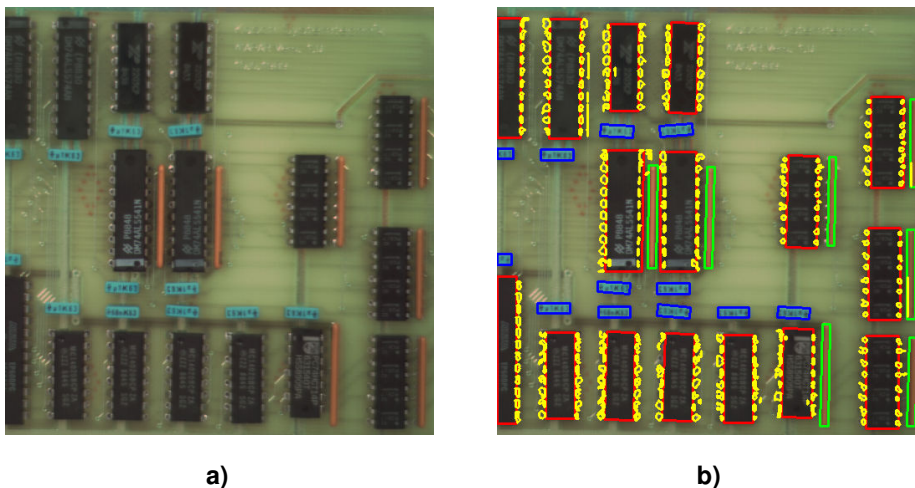
Figure 3.19: (a) Original image; (b) extracted ICs, resistors, and capacitors.
