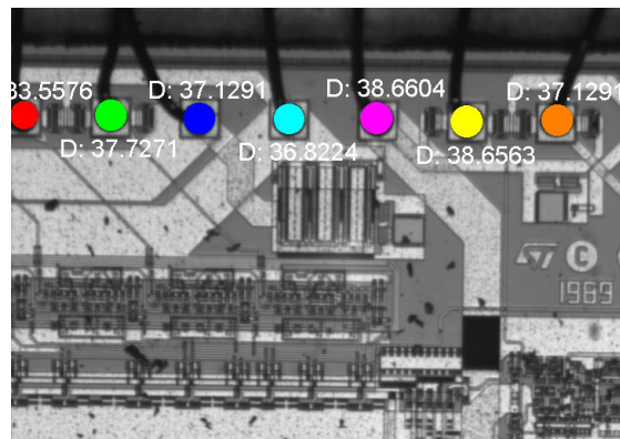
Figure 3.15: Measuring the diameter of ball bonds.
