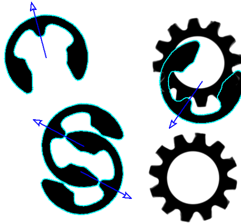
Figure 19: Displaying multiple matches; the used model is depicted in figure 12a on page 22 .
