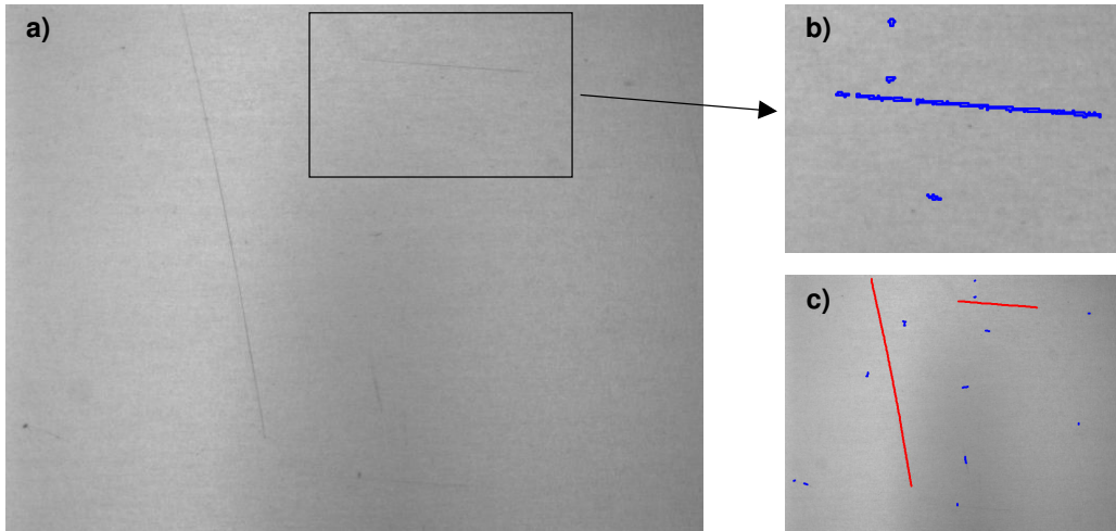
Figure 5.10: Detecting scratches on a metal surface: (a) original image, (b) extracted scratches still partly fractioned, (c) final result with merged scratches.
