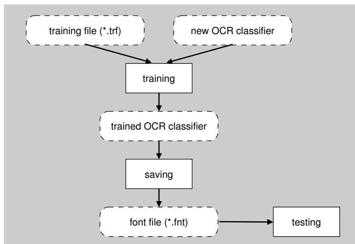
Figure 3.28: Training an OCR classifier.
