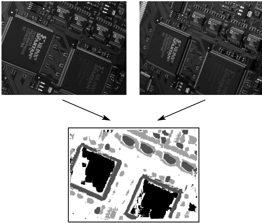
Figure 3.33: Segment board components based on their height.
