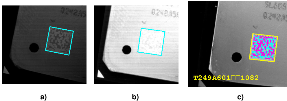
Figure 3.25: (a) Dark training image; (b) bright training image; (c) read code with extracted modules.
