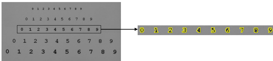
Figure 3.30: Collecting characters for a training file.
