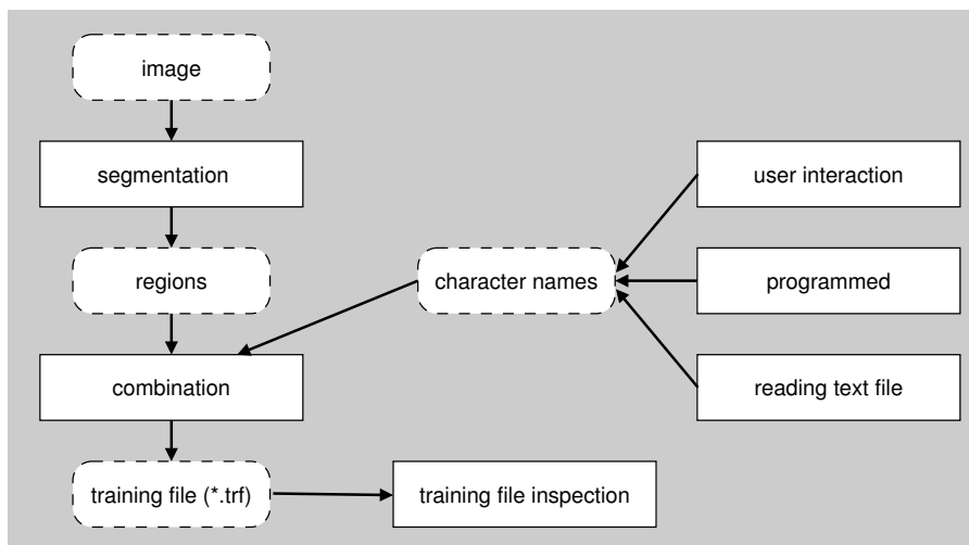
Figure 3.27: Creating training files.
