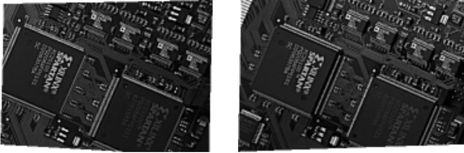
Figure 3.35: Rectified images.
