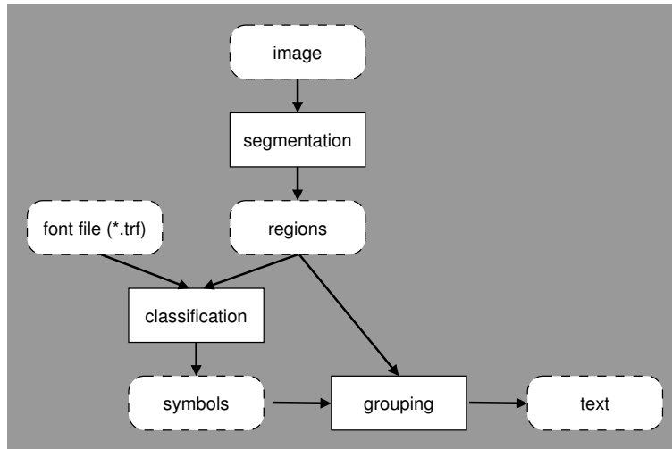
Figure 3.29: Reading characters.
