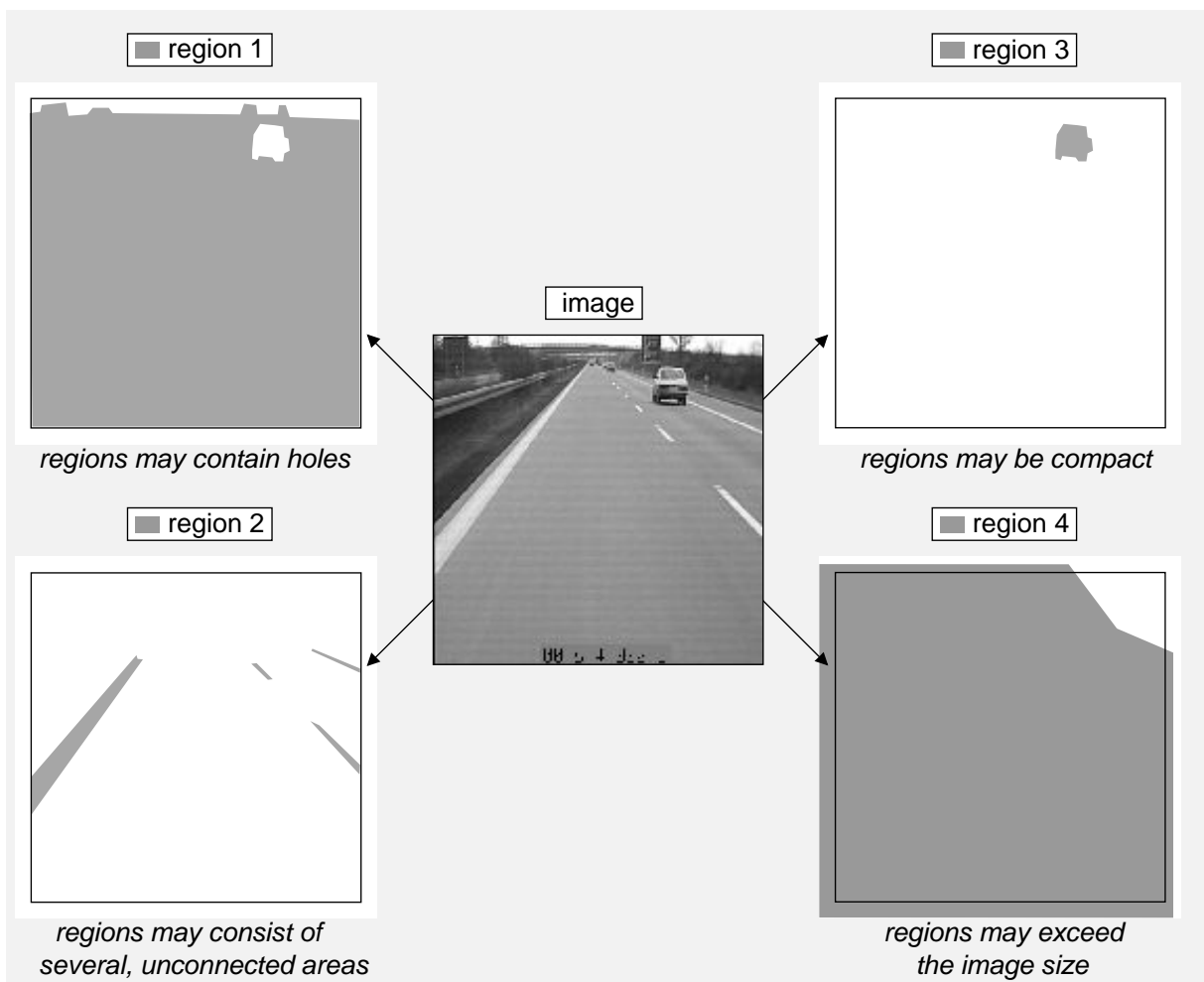
Figure 4.2: Structure of HALCON image objects.
